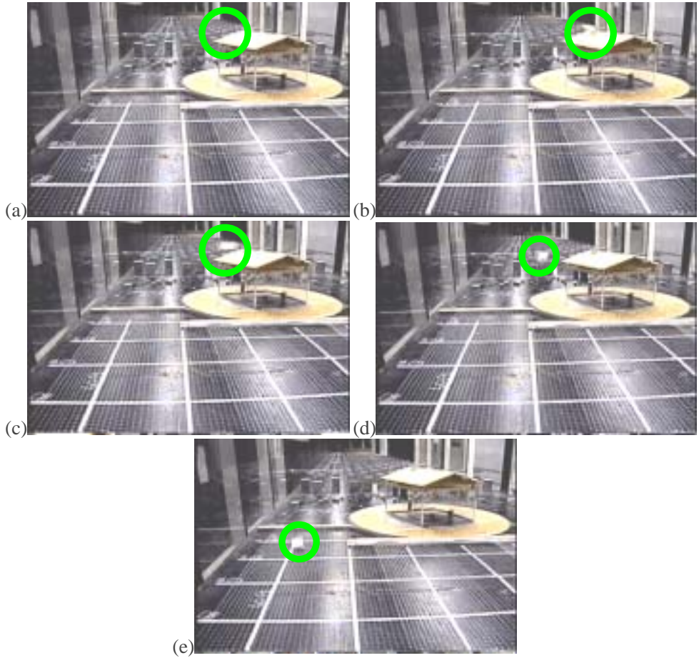
Figure 3. Sequence of images looking upstream showing a failure and trajectory of a 1.2x2.4m (4'x8') sheathing element.
