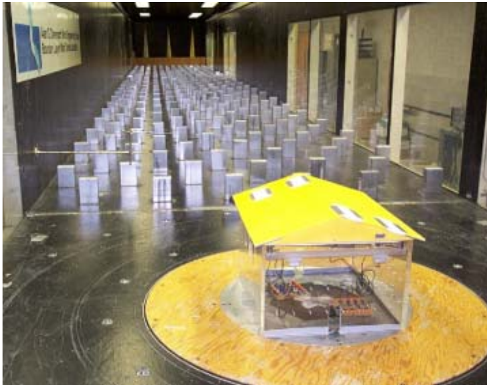
Figure 2. Destructive model in the wind tunnel.
